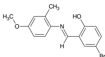
Fig. 1 Primary ligand 4-bromo-2-((E)-[(4-methoxy-2-methylphenyl)imino]methyl)phenol
