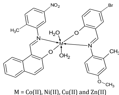
Fig. 4 The metal-ligand ternary binding proposed structure
